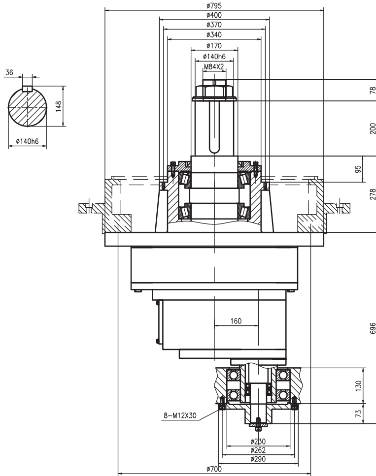
LSJ68 拉丝机专用减速机技术数据 Wire Drawing Machine Gearbox Technical Data
