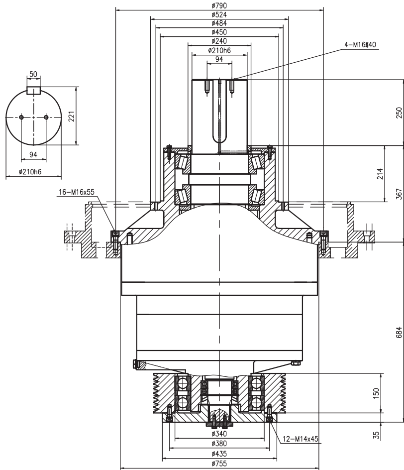
LSJ108 拉丝机专用减速机技术数据 Wire Drawing Machine Gearbox Technical Data
