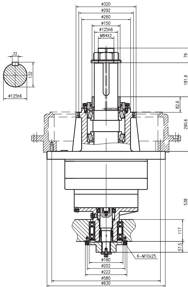
LSJ48 拉丝机专用减速机技术数据 Wire Drawing Machine Gearbox Technical Data
