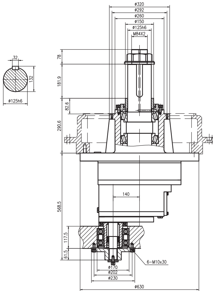
LSJ48 拉丝机专用减速机技术数据 Wire Drawing Machine Gearbox Technical Data
