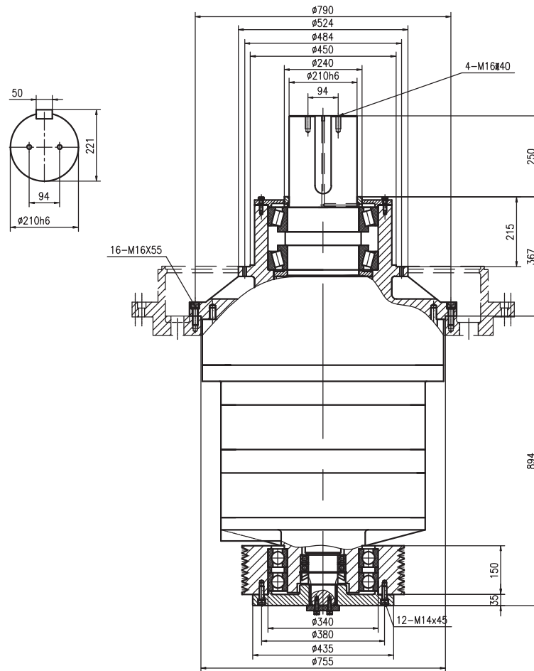
LSJ108 拉丝机专用减速机技术数据 Wire Drawing Machine Gearbox Technical Data
