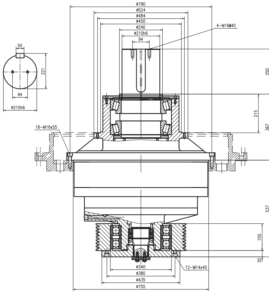
LSJ108 拉丝机专用减速机技术数据 Wire Drawing Machine Gearbox Technical Data
